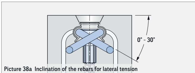
Picture 38a Inclination of the rebars for lateral tension
