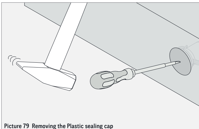
Picture 79 Removing the Plastic sealing cap
